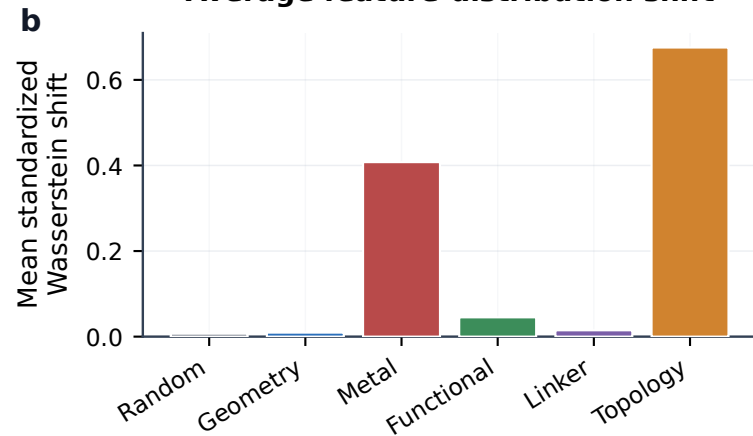
Average feature-distribution shift
