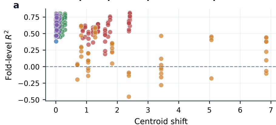
Descriptor-space displacement vs performance
