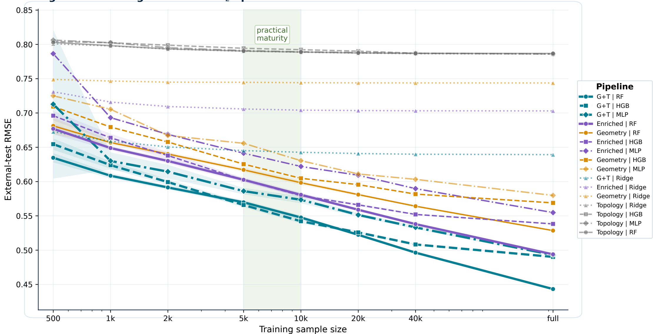
Figure 2. Learning curves for CO 2 uptake at 0.15 bar
