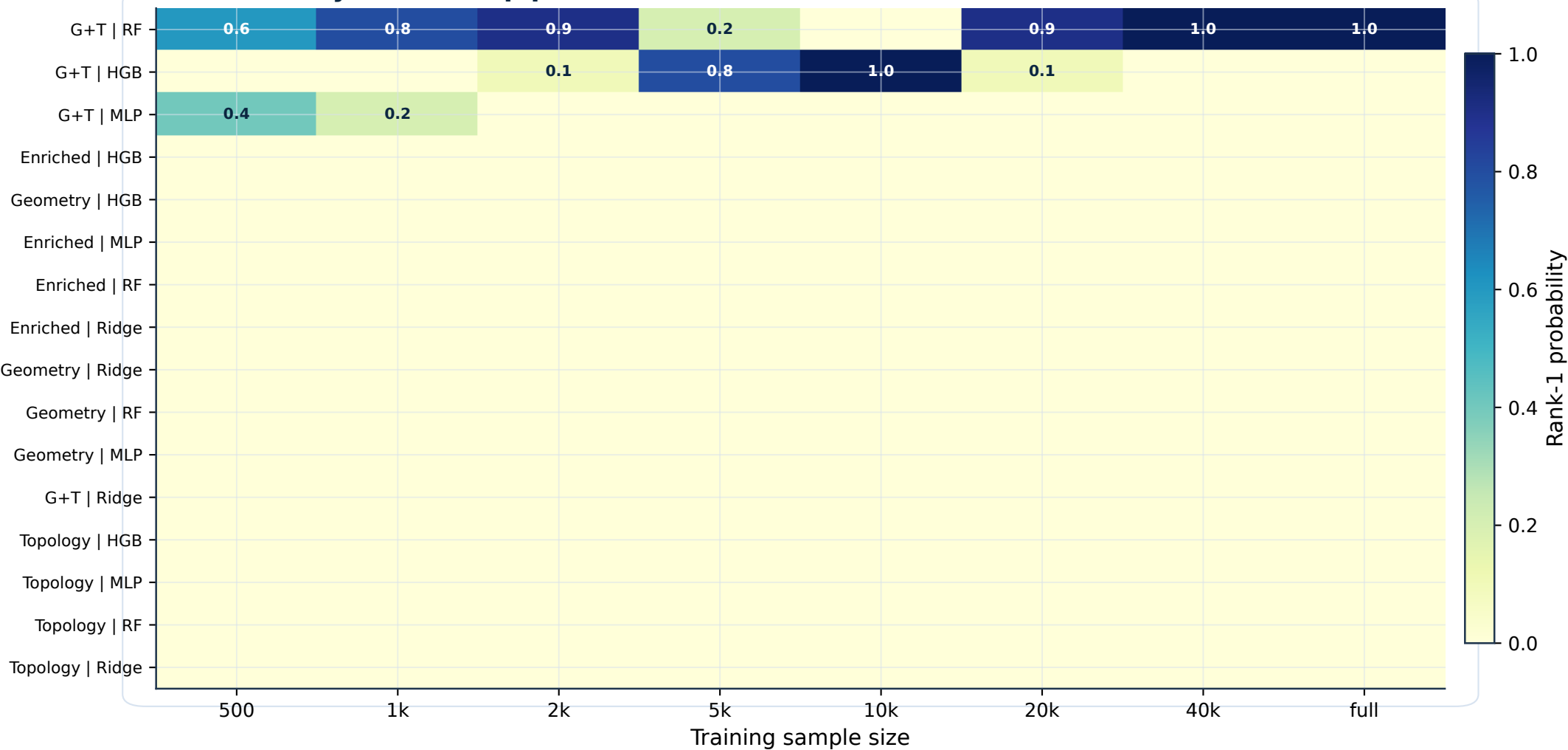
a Probability that each pipeline ranks first
