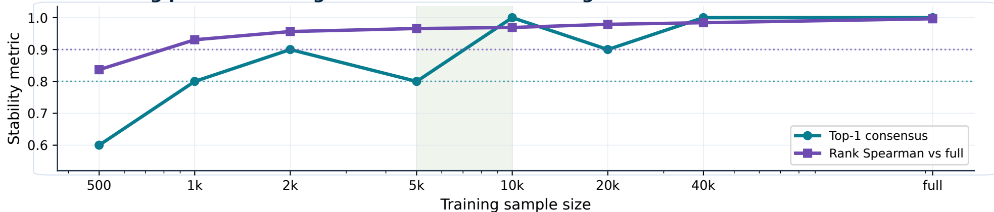
b Ranking preservation against the full-data ordering
