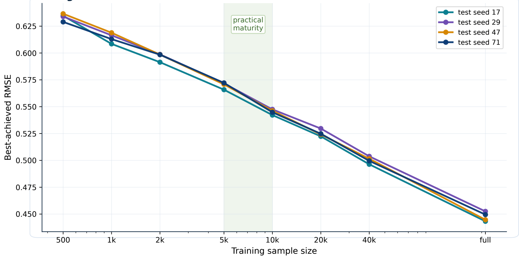
SI Figure 1. Robustness across fixed external test sets
