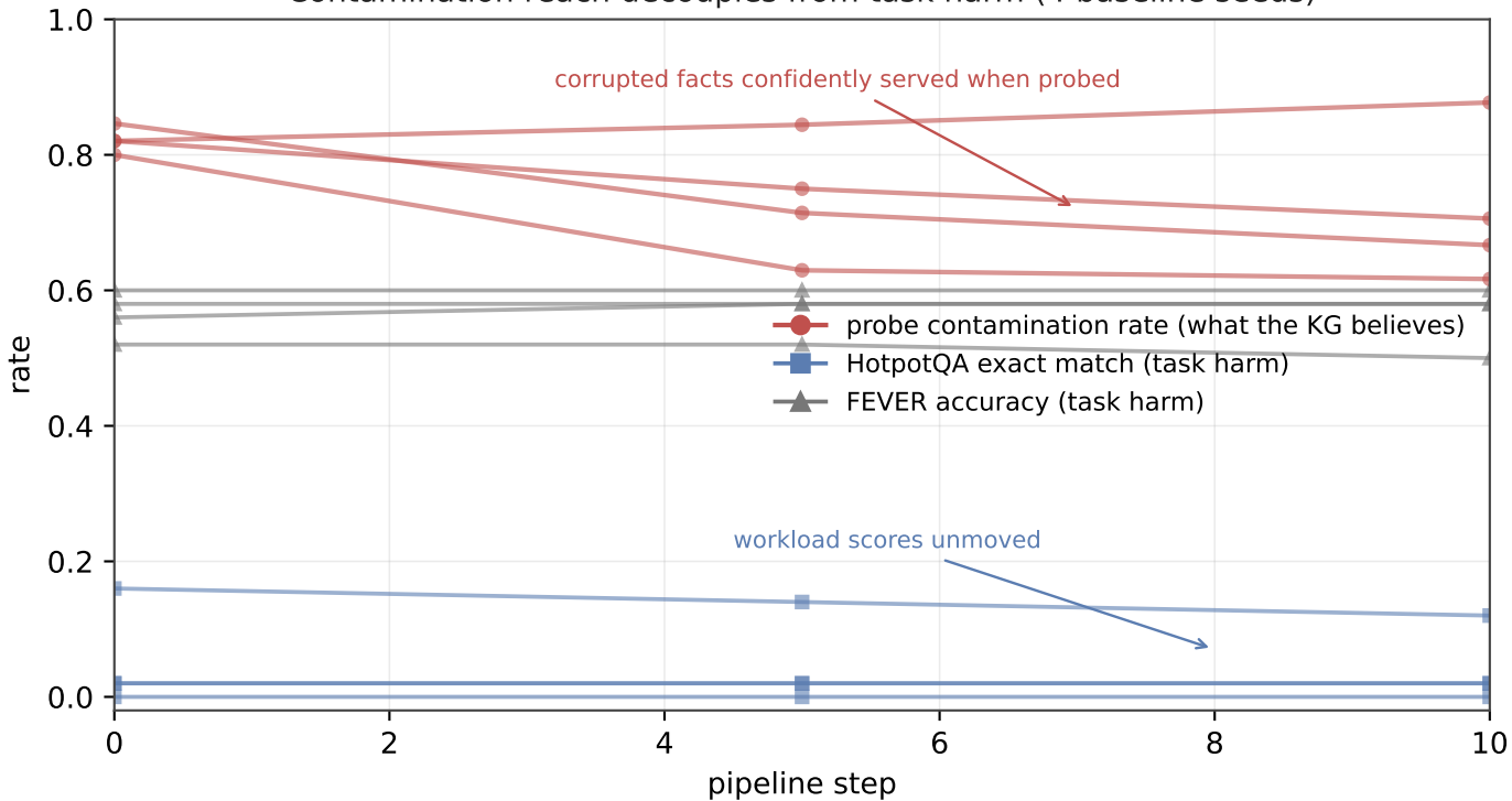
Contamination reach decouples from task harm (4 baseline seeds)
