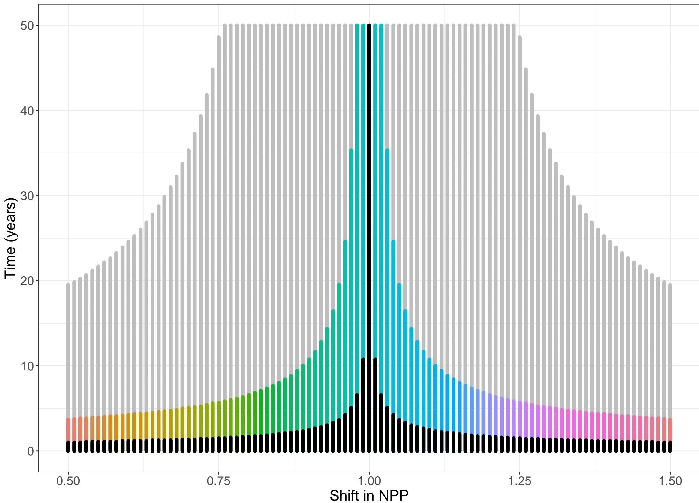
Accuracy of One-Pool to Five-Pool model within 10%, 1%, and 0.1% of original steady state
