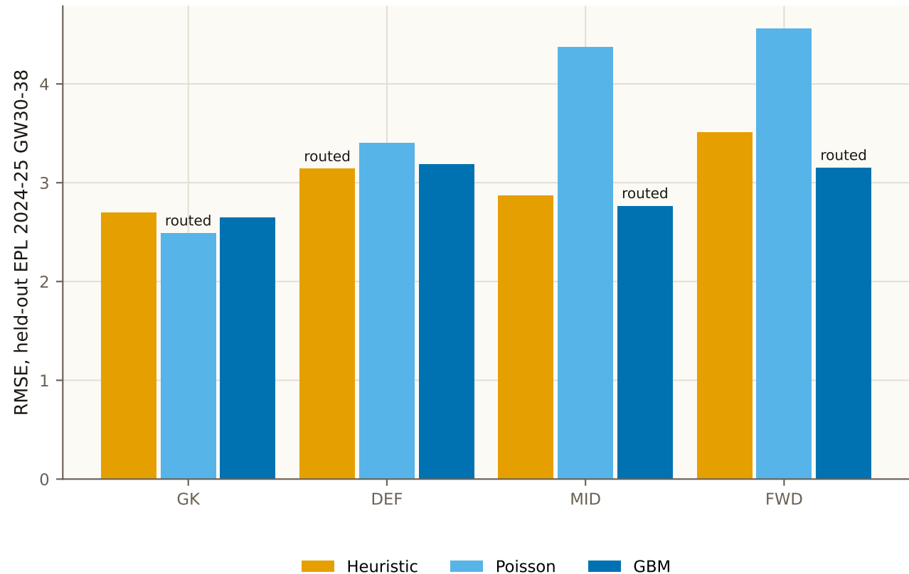
Held-out accuracy by position; the ensemble routes each position to its winner
