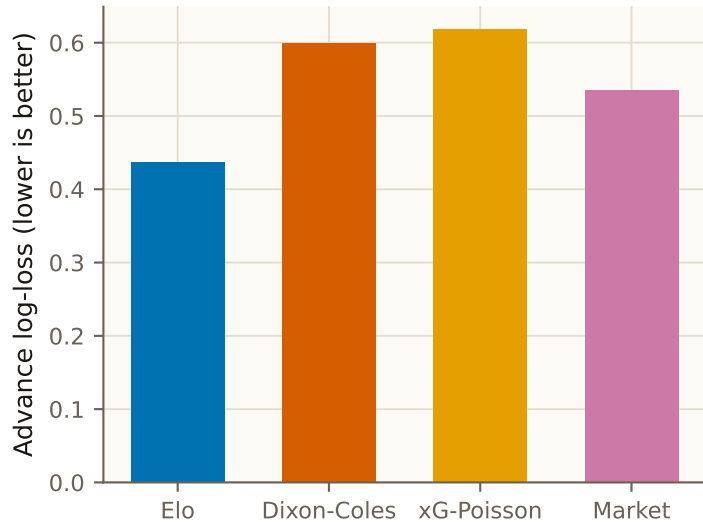
Knockout advance skill, rounds 4-7
