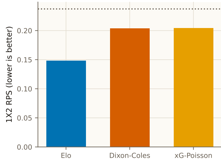
90-minute outcome skill, held-out rounds 2-7
