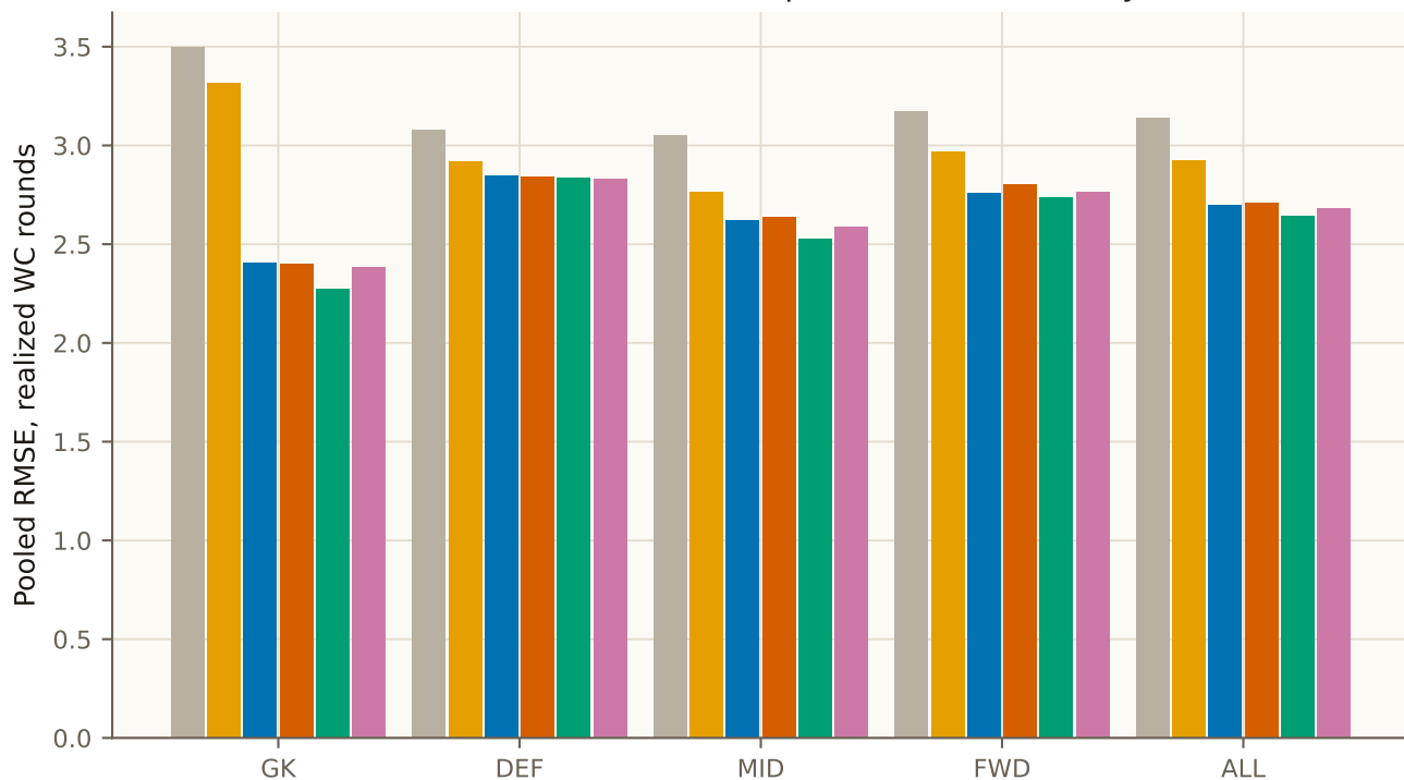
Walk-forward validation on realized World Cup rounds (train strictly before each round)
