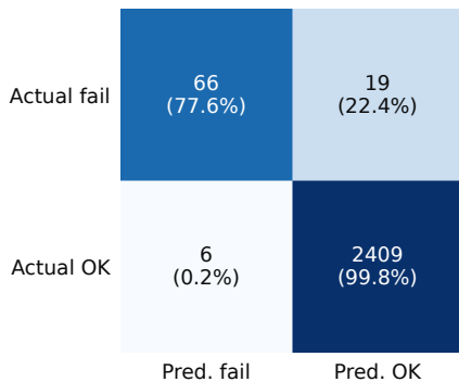
RF
