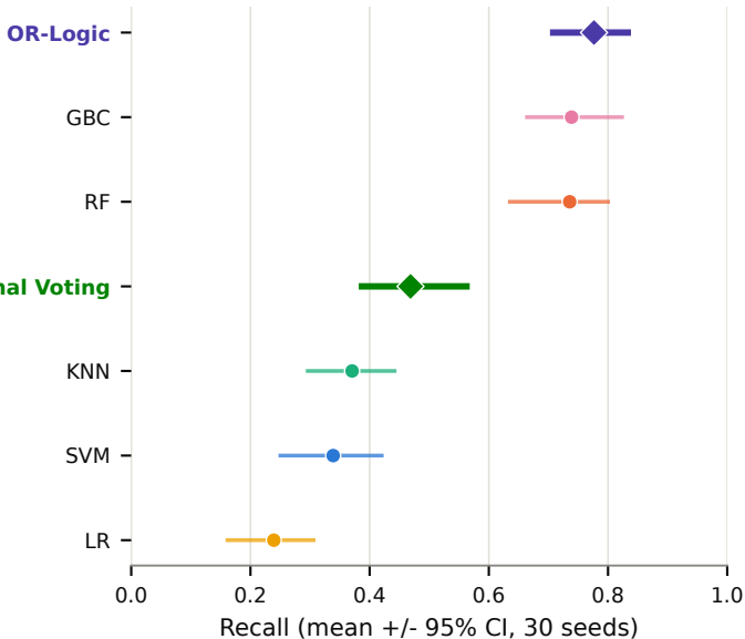
Recall stability across 30 seeds
