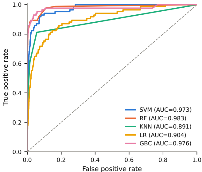
ROC -- base models, modified features (SEED=42)
