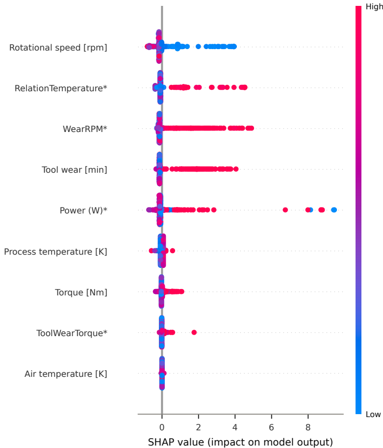
SHAP beeswarm -- GBC
