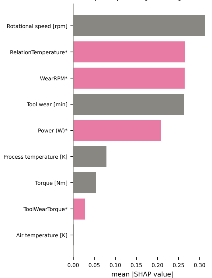
Mean |SHAP| ranking (* = engineered)
