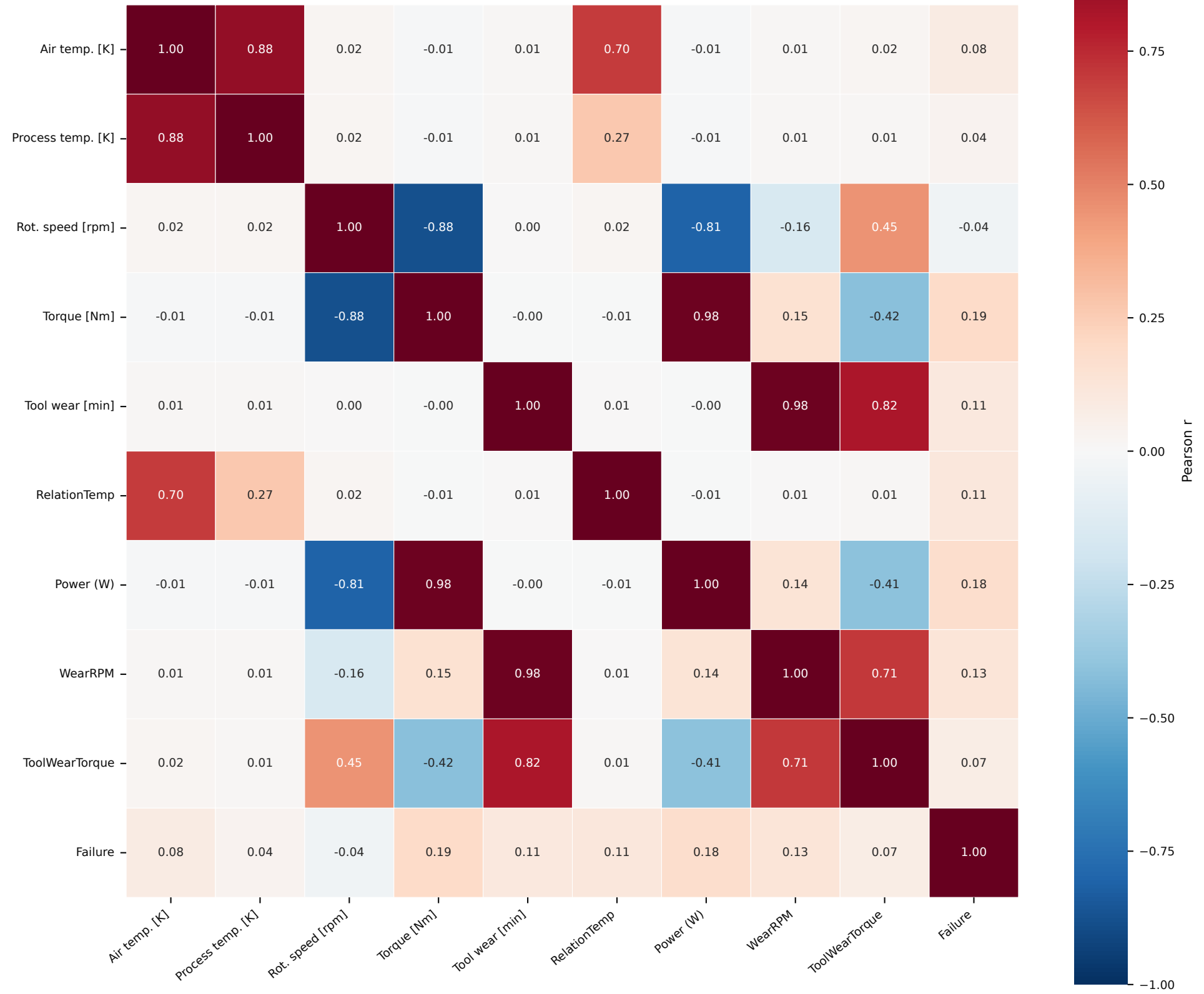
Correlation matrix -- original + engineered features
