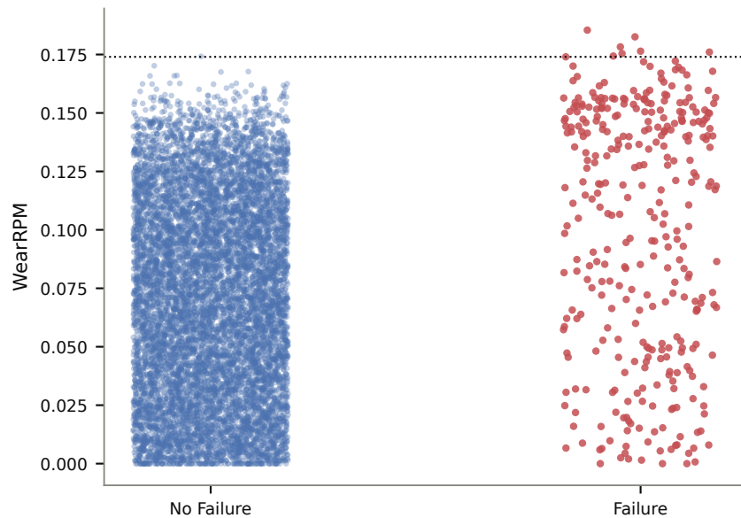
WearRPM (claimed threshold 0.174)
