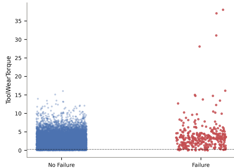
ToolWearTorque (claimed threshold 0.26253)
