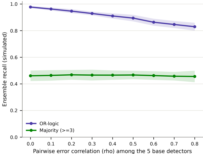
OR-logic vs. majority-voting recall vs. detector correlation
