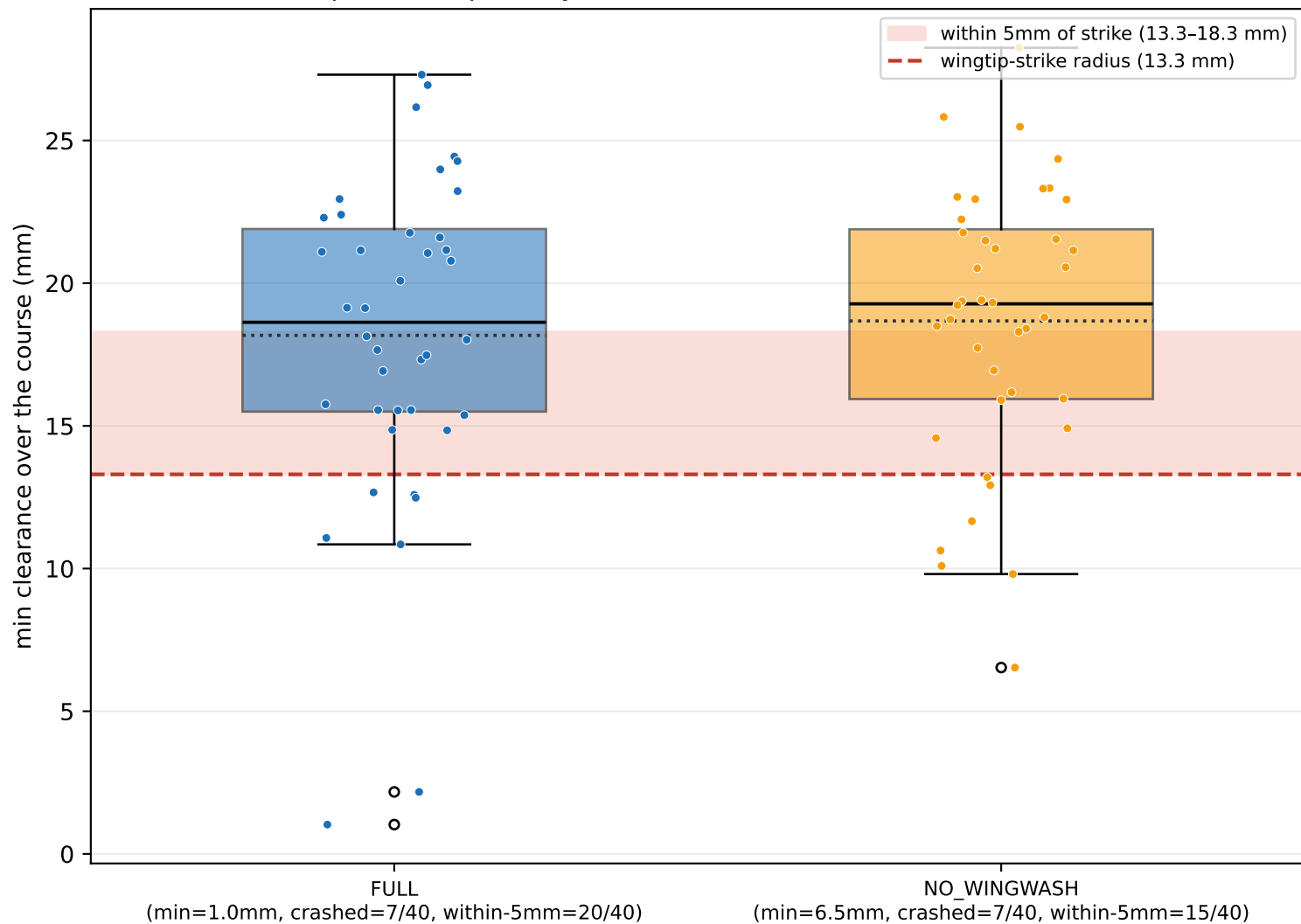
Per-course minimum clearance: FULL vs NO_WINGWASH (e51b part1, 40 primary courses, level=1.0 noise, rate=1000 Hz)
