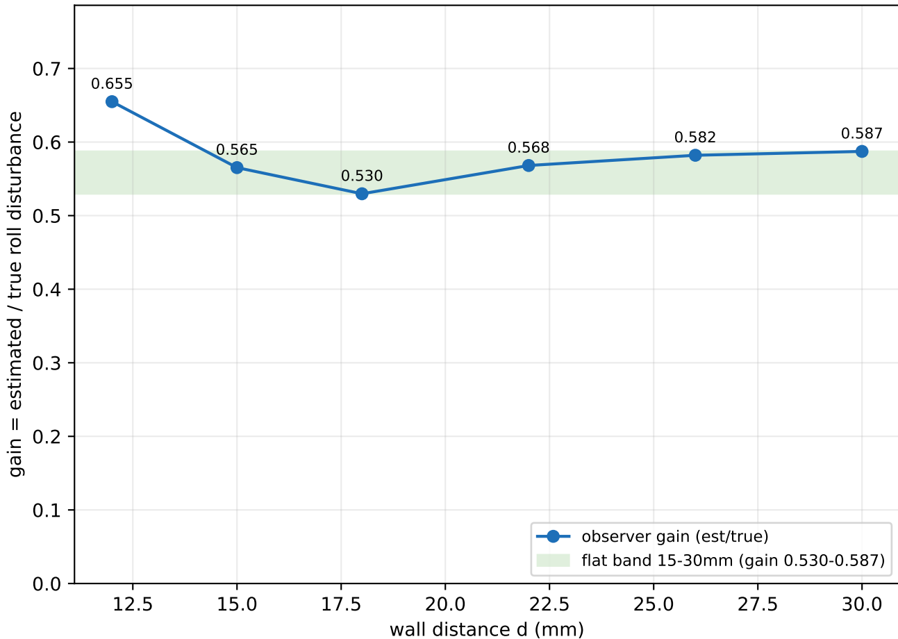
Disturbance-observer fidelity: gain vs wall distance (rise time 10-90% = 13.0 ms, step response trace not in committed CSV)
