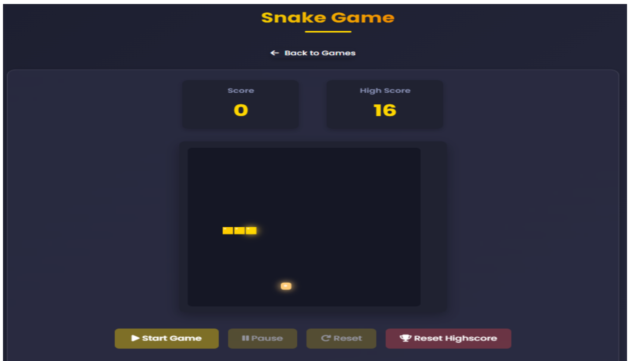
Figure 10: Snake Game
