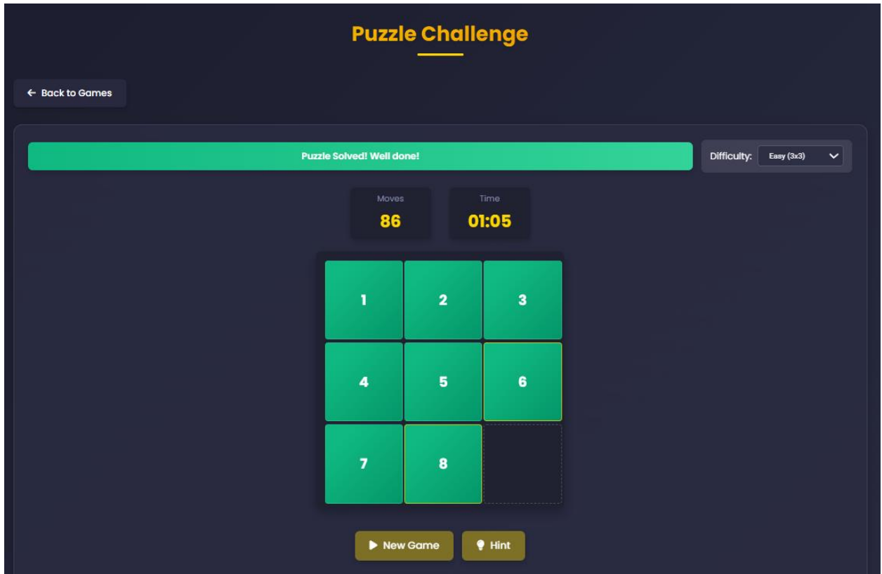
Figure 11: Puzzle Game
