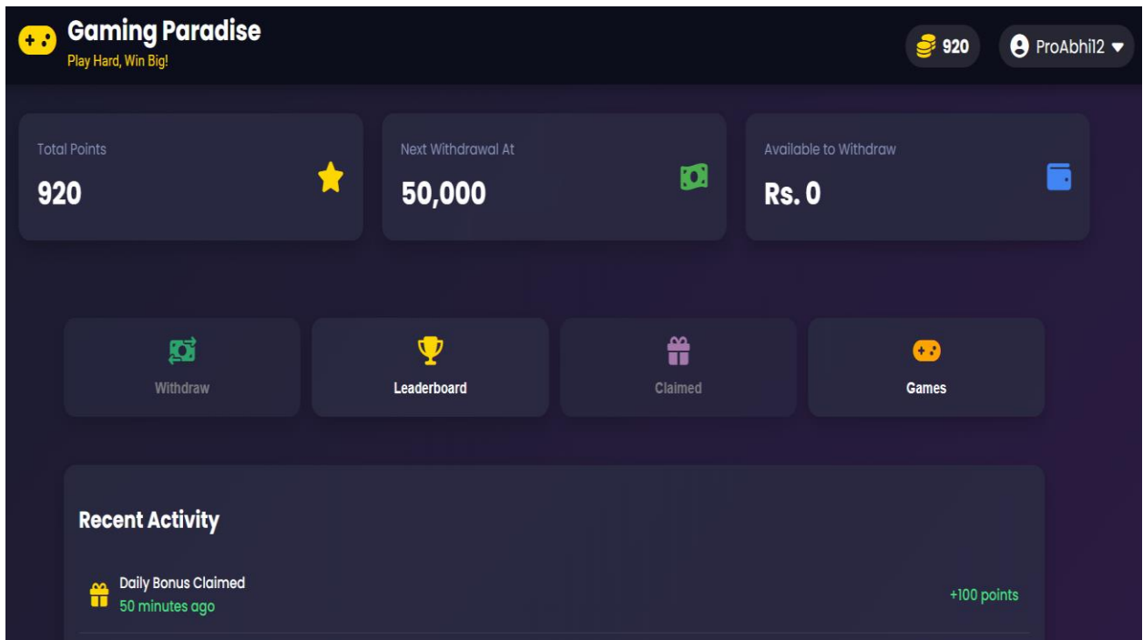
Figure 7: Dashboard Page
