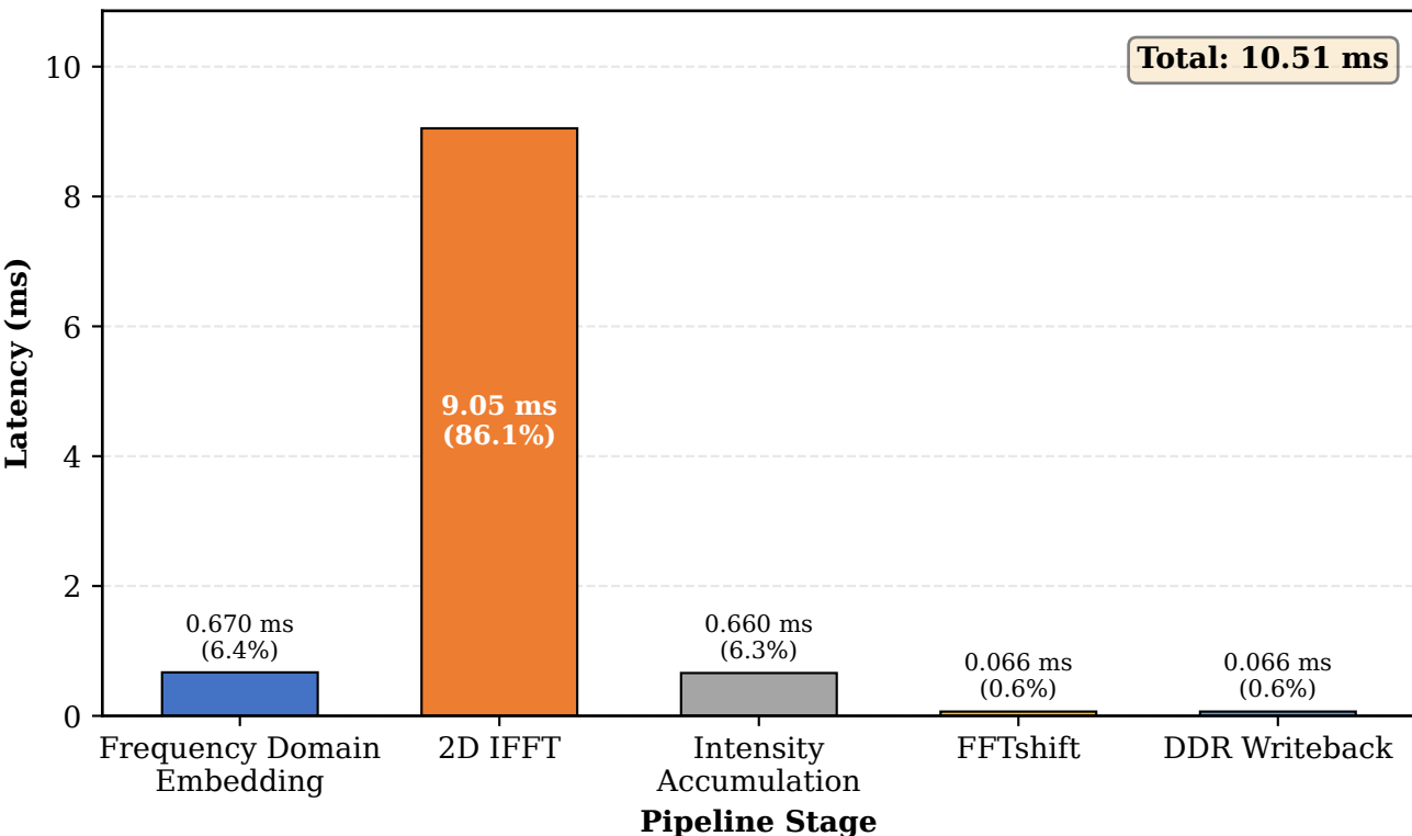
Figure 5-2: Latency Breakdown of Single SOCS Imaging (@ 250 MHz)
