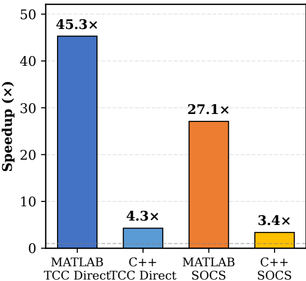
(a) FPGA Speedup vs CPU Baselines
