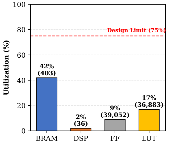
(b) Resource Utilization on xcku5p
