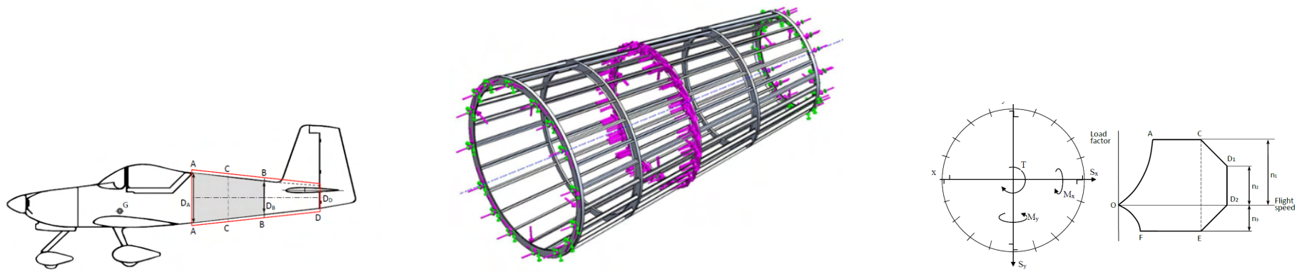
Figure 6: Rear fuselage geometry, loading, and stringer stress distribution
