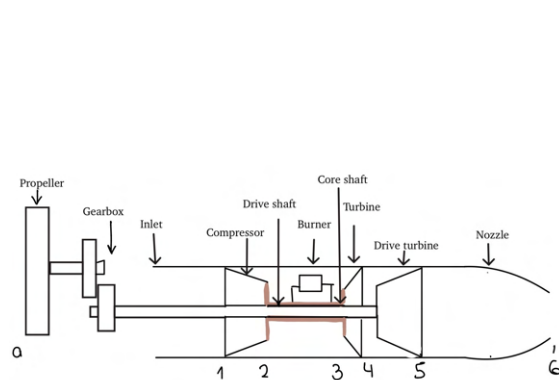
Figure 3: Gas turbine cycle and propeller performance evaluation
