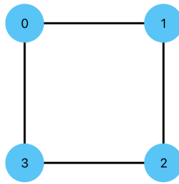
Figure 6.1: case 1 |0000\rangle [3]
