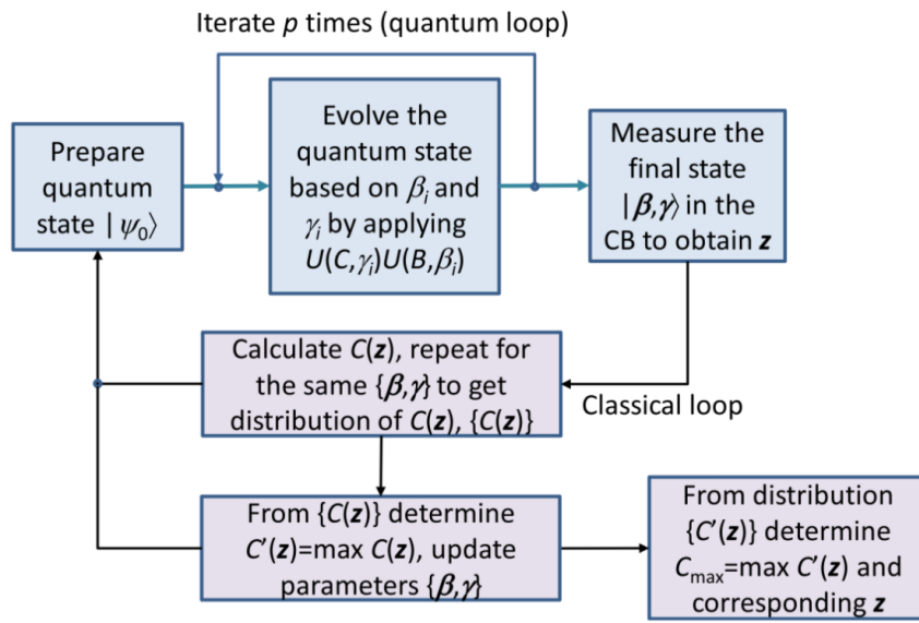
Figure 4.3: QAOA procedure [1].
