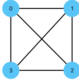
Figure 6.5: Case 2 |0000\rangle
