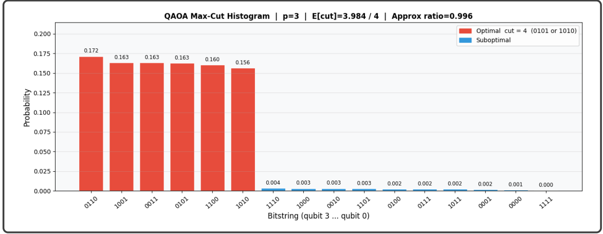
Figure 6.7: Results of 8192 shots for case 2, p = 3 . [3]
