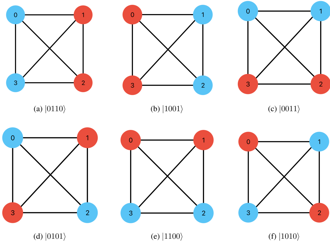
Figure 6.8: Solutions to case 2 of the Max-Cut problem.
