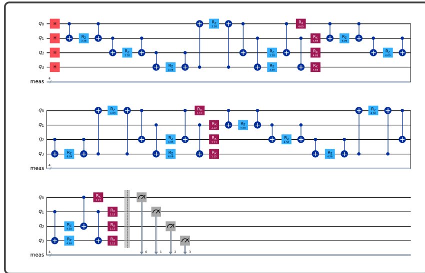
Figure 6.6: Circuit for QAOA application on a square grid with n=4 and edges = 6 and p = 3 [3].
