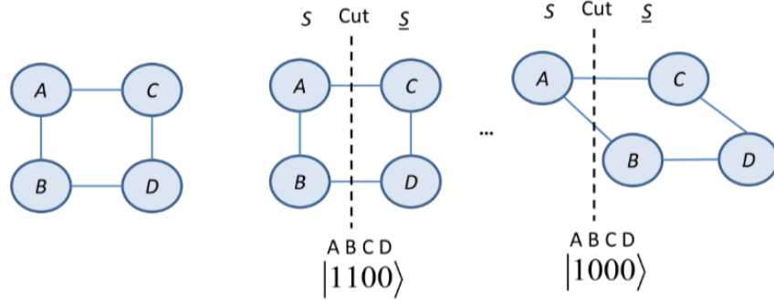
Figure 5.1: Max-Cut problem [1].
