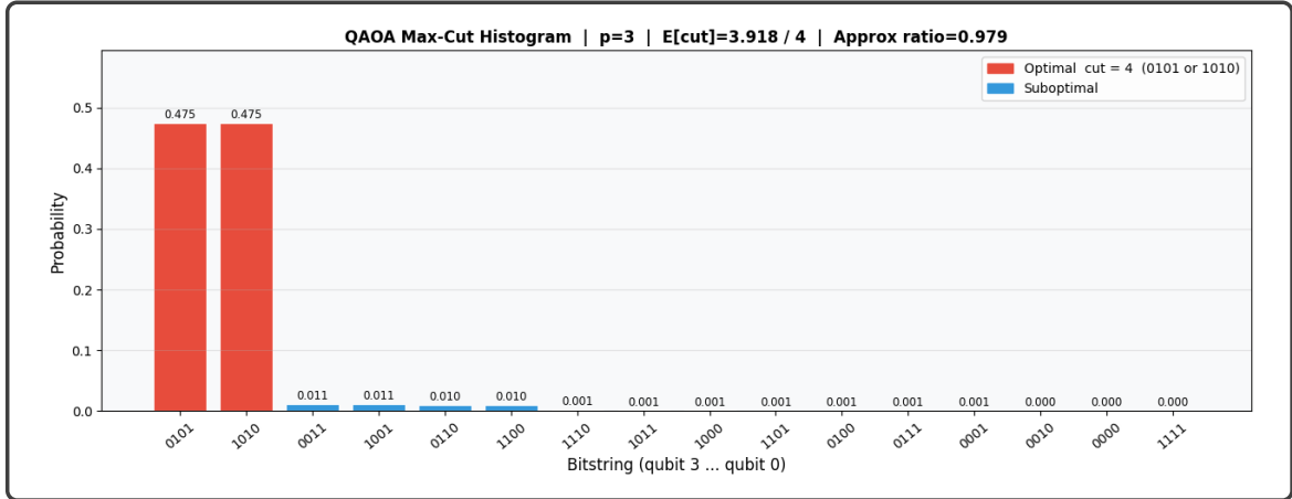
Figure 6.3: Results of 8192 shots for case 1, p = 3 . [3]
