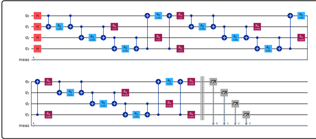
Figure 6.2: Circuit for QAOA application on a square grid with p = 3 [3].
