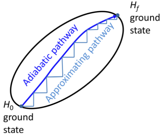
Figure 4.2: Approximation of the adiabatic pathway [1].
