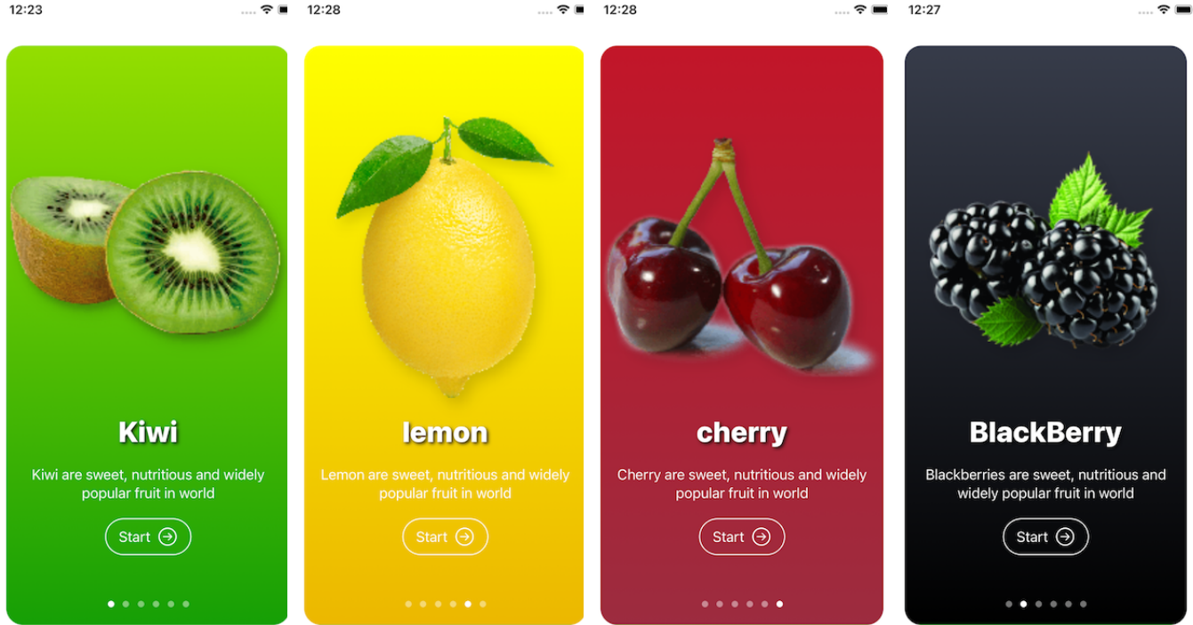
Onboarding UI
