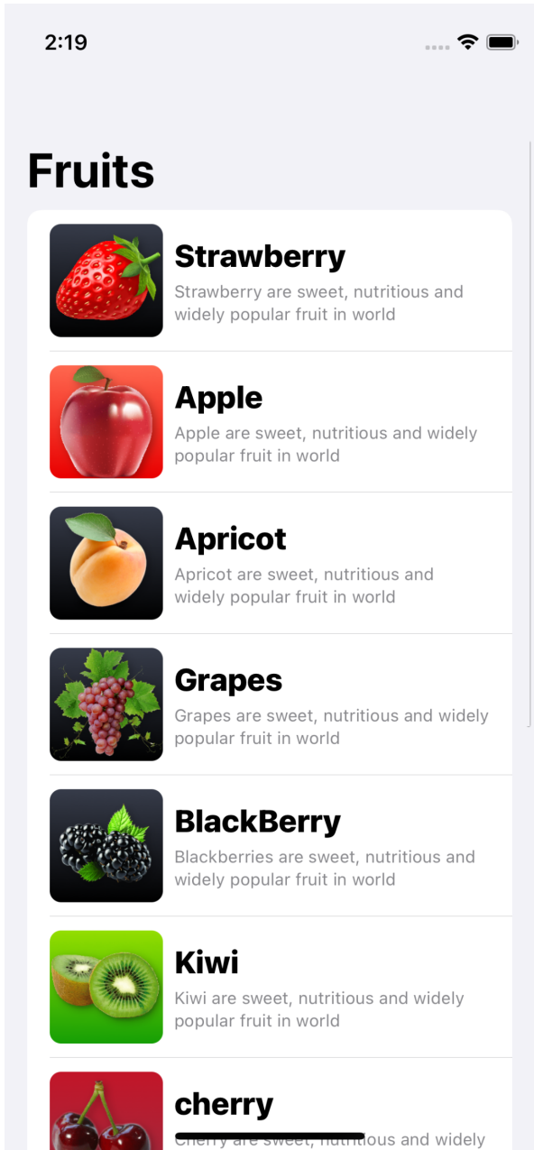
Dashboard UI
