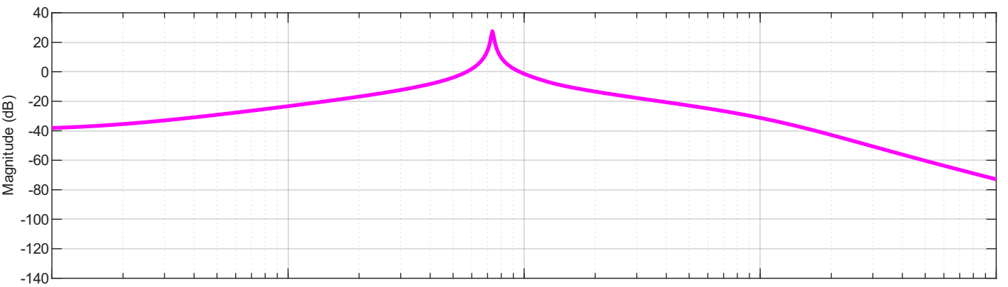
Minor-loop gain T_m = Z_o/Z_i (diagnostic only)
