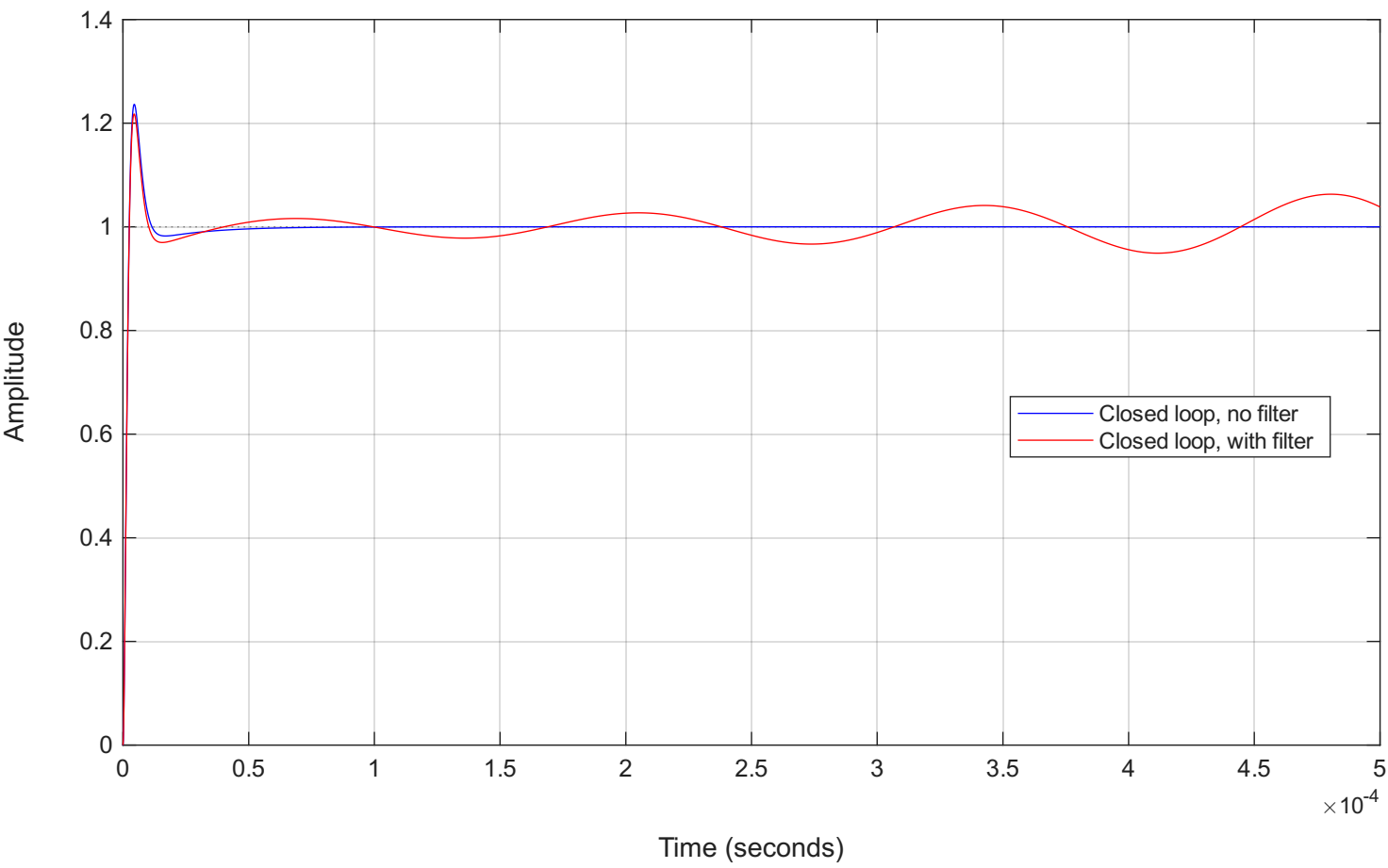
Closed-loop step response: no filter (blue) vs with filter (red)
