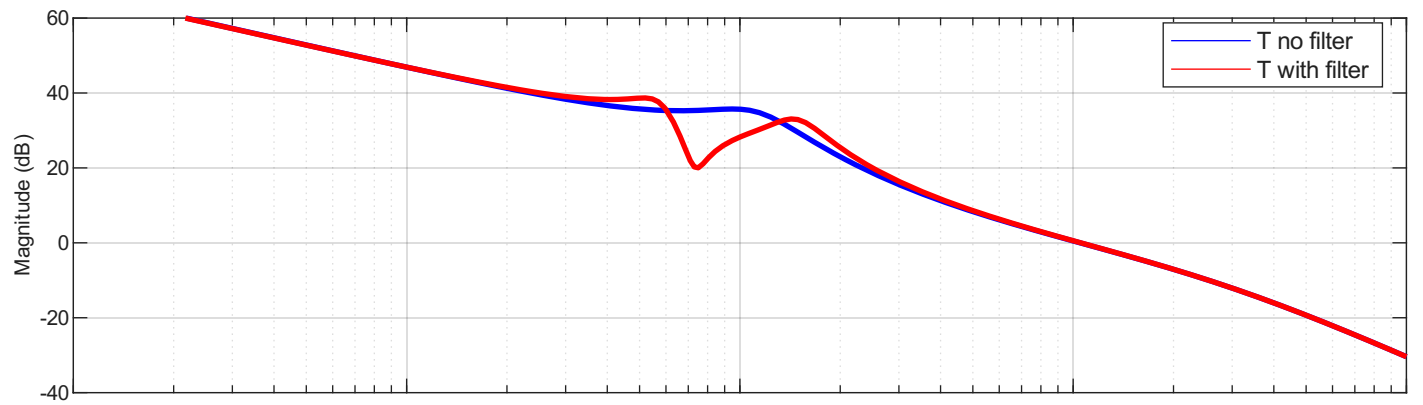
Loop gain T: no filter (blue) vs with input filter (red)
