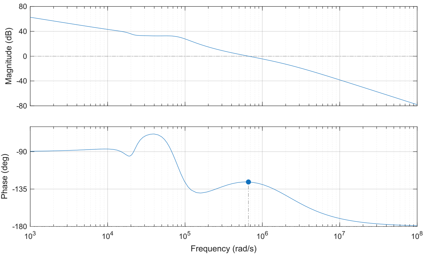
Damped filter ( R_d=0.143\Omega ): loop gain margin Gm = Inf, Pm = 53.5 deg (at 6.6\text{e}+05 rad/s)
