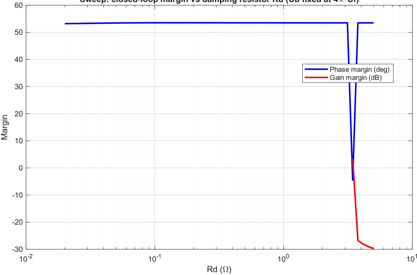
Sweep: closed-loop margin vs damping resistor R_d ( C_b fixed at 4 \times C_f )
