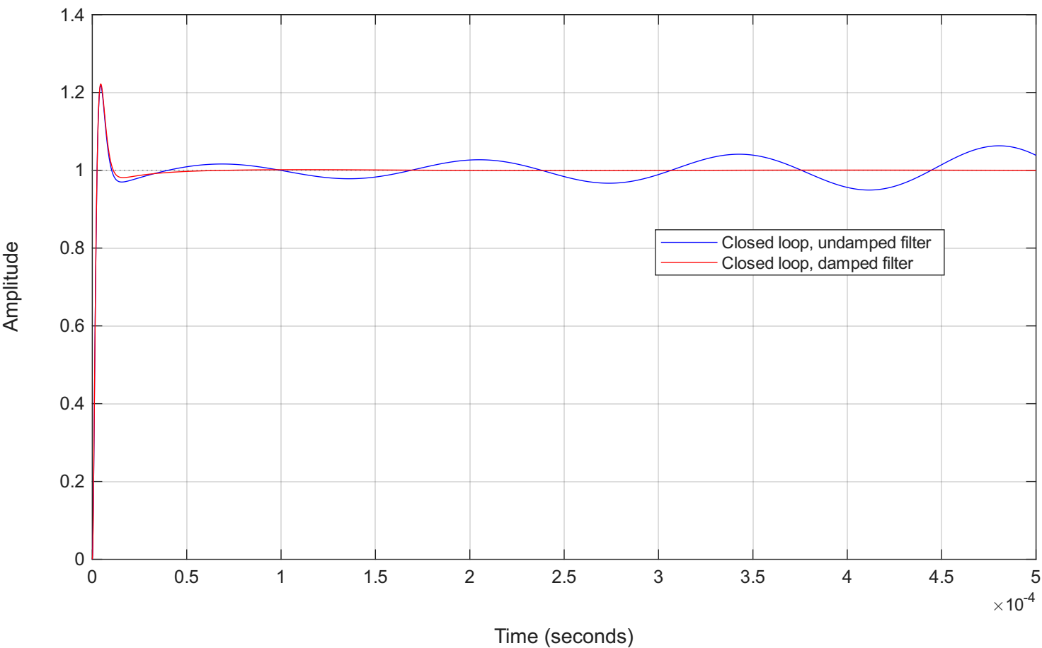
Step response: undamped (blue, ringing) vs damped (red)
