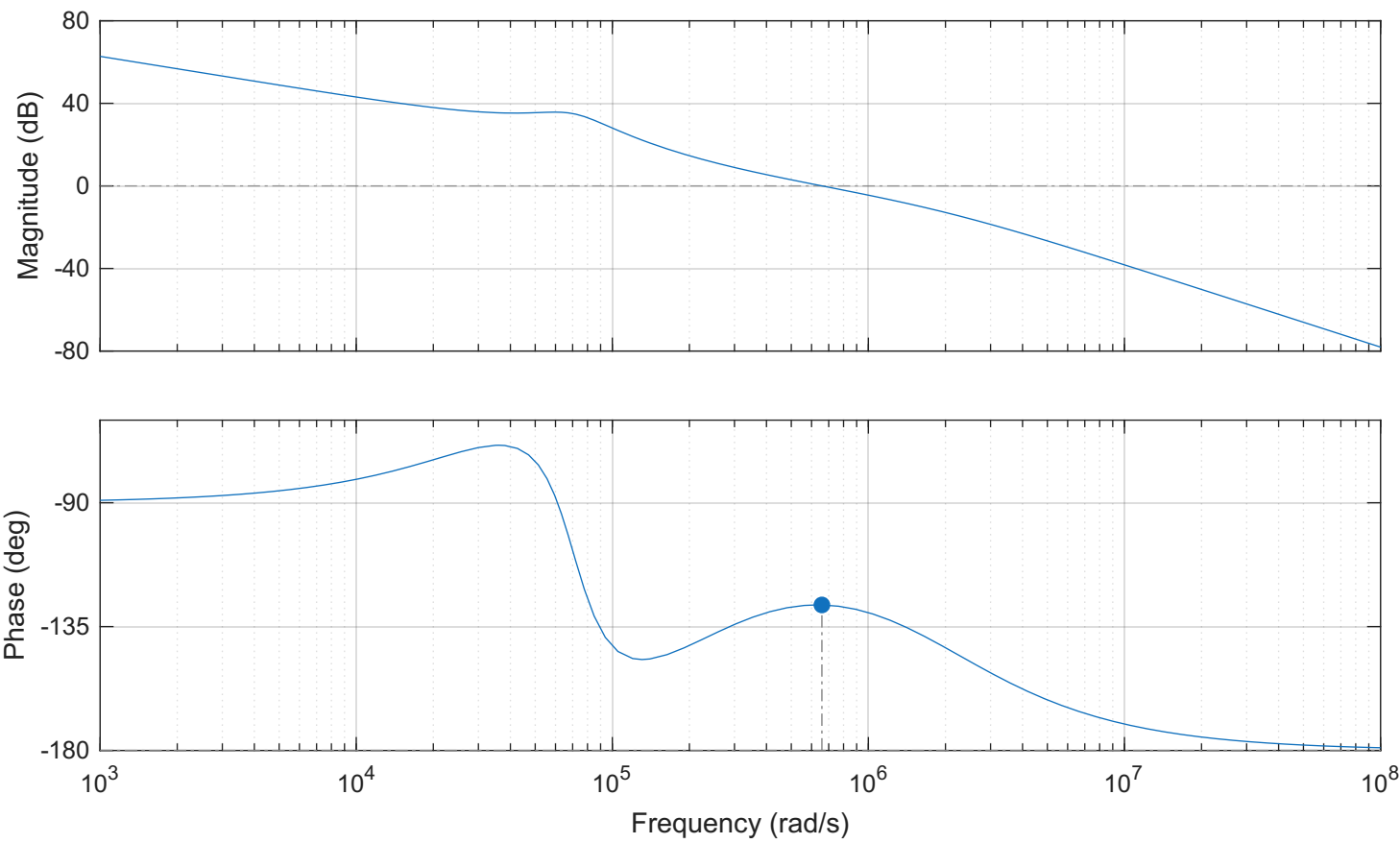
Converter alone: loop gain T, margin plot (baseline) Gm = Inf, Pm = 52.9 deg (at 6.58e+05 rad/s)
