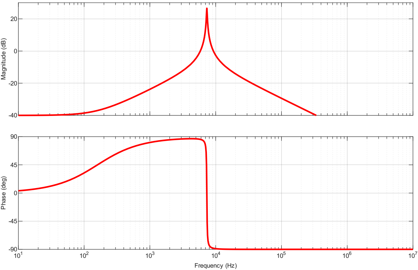
Filter output impedance Z_o (standalone)
