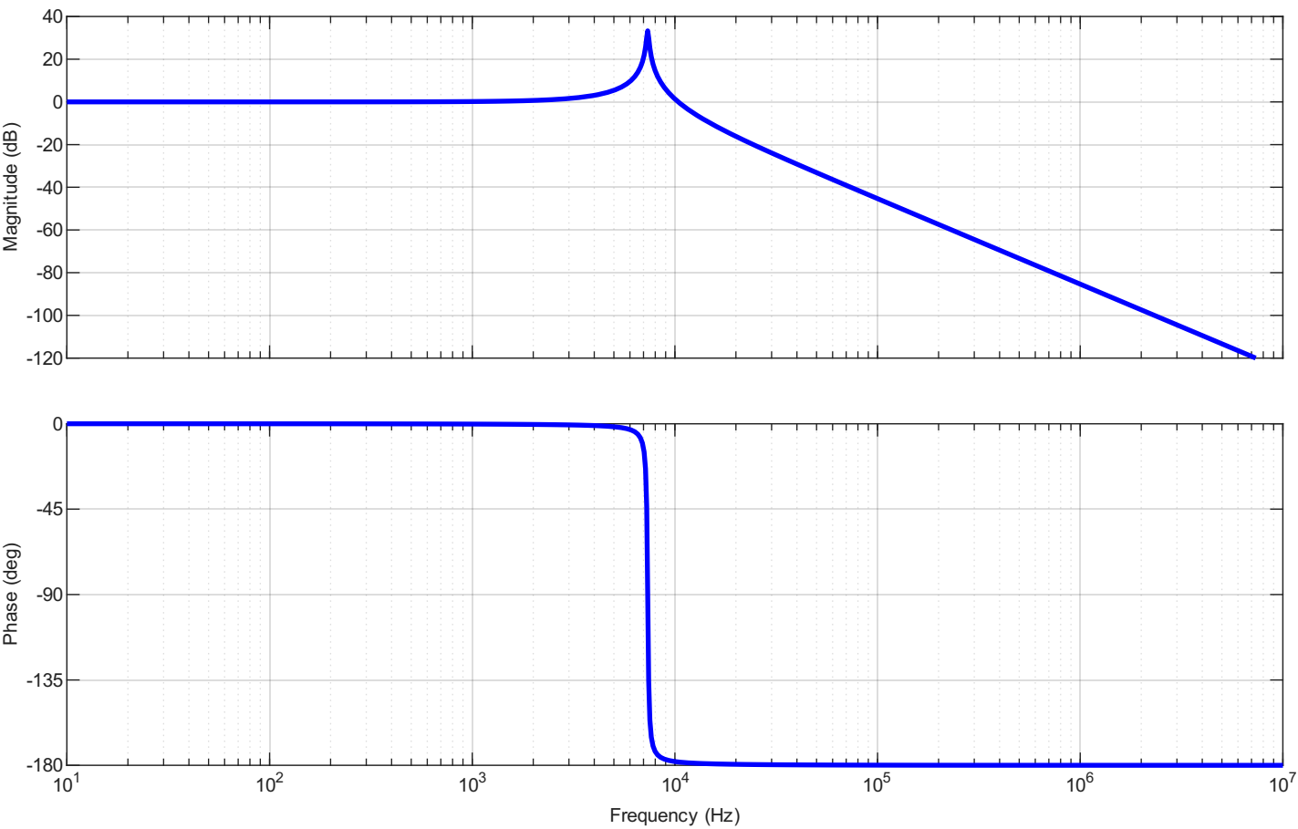
Filter frequency response (standalone, unloaded)
