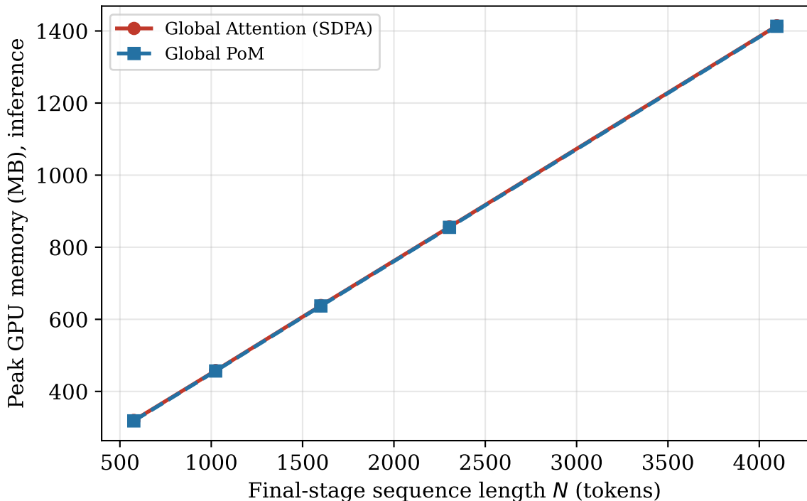
Inference peak memory is identical (SDPA hides the matrix)
