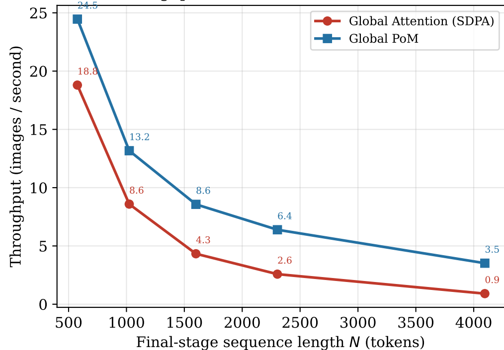
(a) Throughput vs. token count (MambaVision-T)
