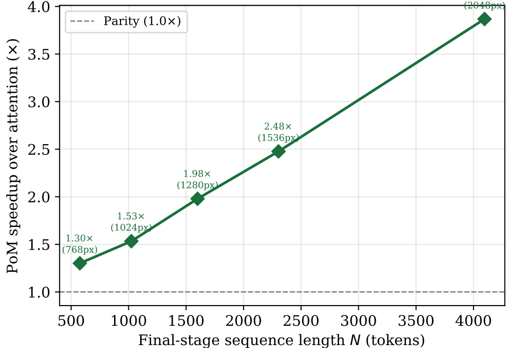
(b) Relative speedup grows with N
