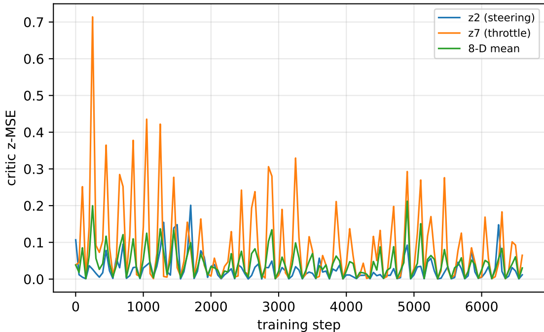
Critic egomotion-prediction error
