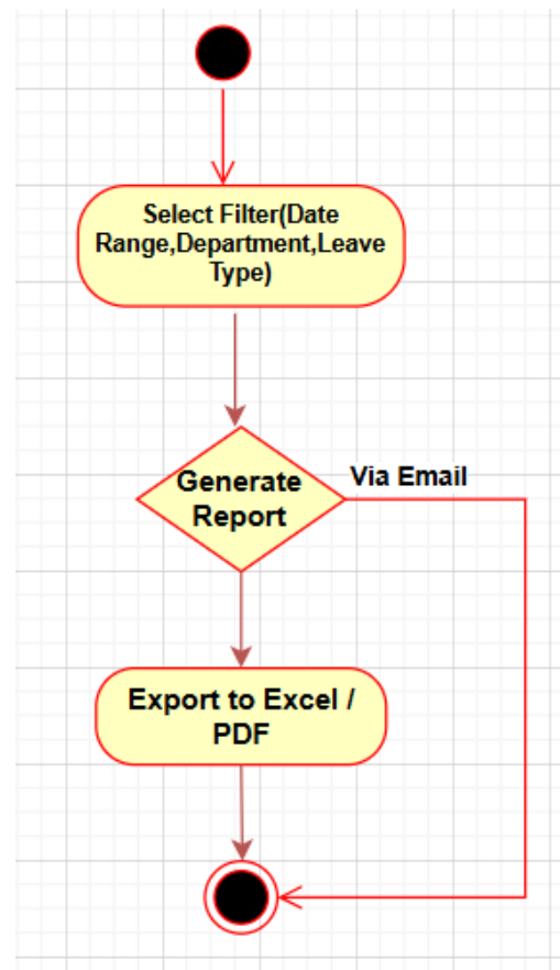
Figure 6: Generate Leave Reports (HR) – Activity Flow
