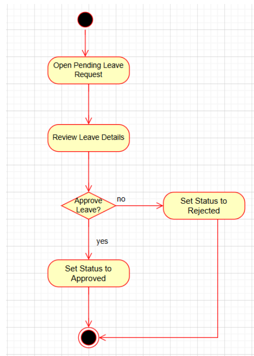
Figure 2: Manager Approves or Rejects Leave – Activity Flow
