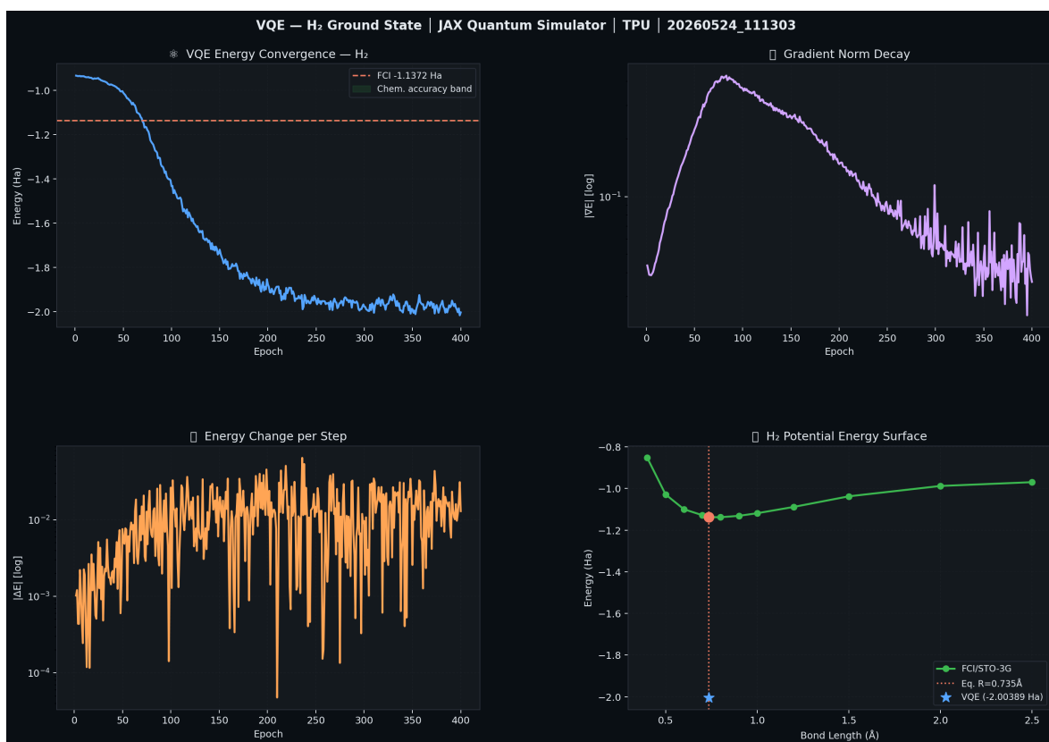
Figure 3: VQE H_2 molecular simulation. Top-left: energy convergence toward FCI reference (dashed red). Green shaded band marks chemical accuracy ( \pm 1.6 mHa). Top-right: gradient norm decay. Bottom-right: H_2 potential energy surface with FCI curve (green) and VQE result (star marker).
