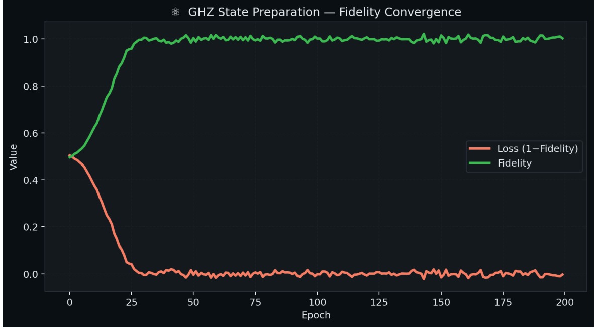
Figure 1: GHZ State Preparation — Fidelity and loss convergence over 200 Adam epochs on GPU (RTX 2050). Orange: infidelity (loss, 1 - F ); Green: state fidelity F . Both GPU and TPU executions achieve identical final fidelity.
