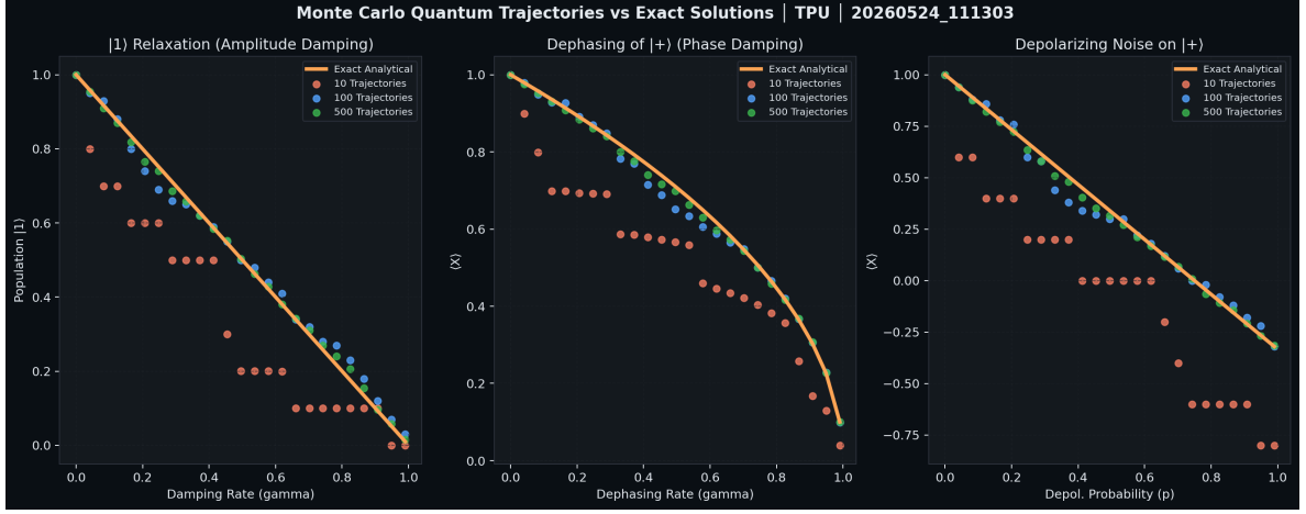
Figure 7: Monte Carlo quantum noise simulation. Left: amplitude damping |1\rangle relaxation vs damping rate \gamma . Center: phase damping \langle X \rangle decay of |+\rangle . Right: depolarizing channel \langle X \rangle decay. Yellow curve: exact analytical solution. Colored markers: 10/100/500-trajectory Monte Carlo averages converging to exact solutions.
