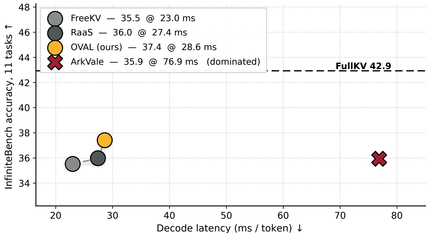
Accuracy vs. latency — Llama-3.1-8B-Instruct, B = 2048 , 32K input
