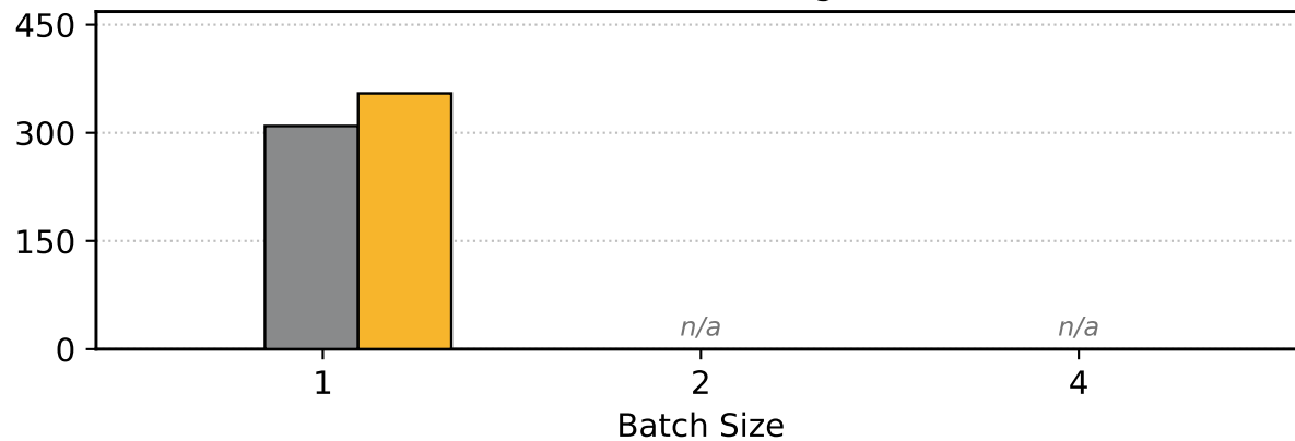
Llama-3.1-8B-Instruct (Long Generation)
