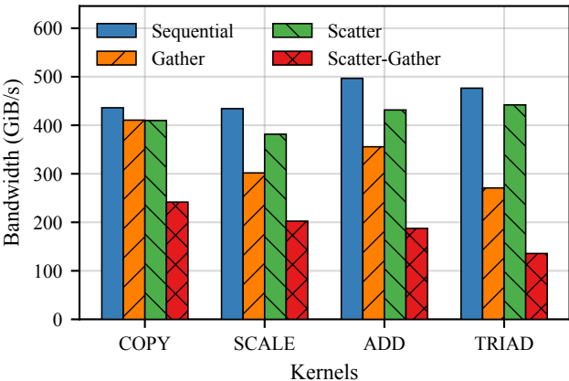
Bandwidth across Access Patterns (N=131072, L=40)
