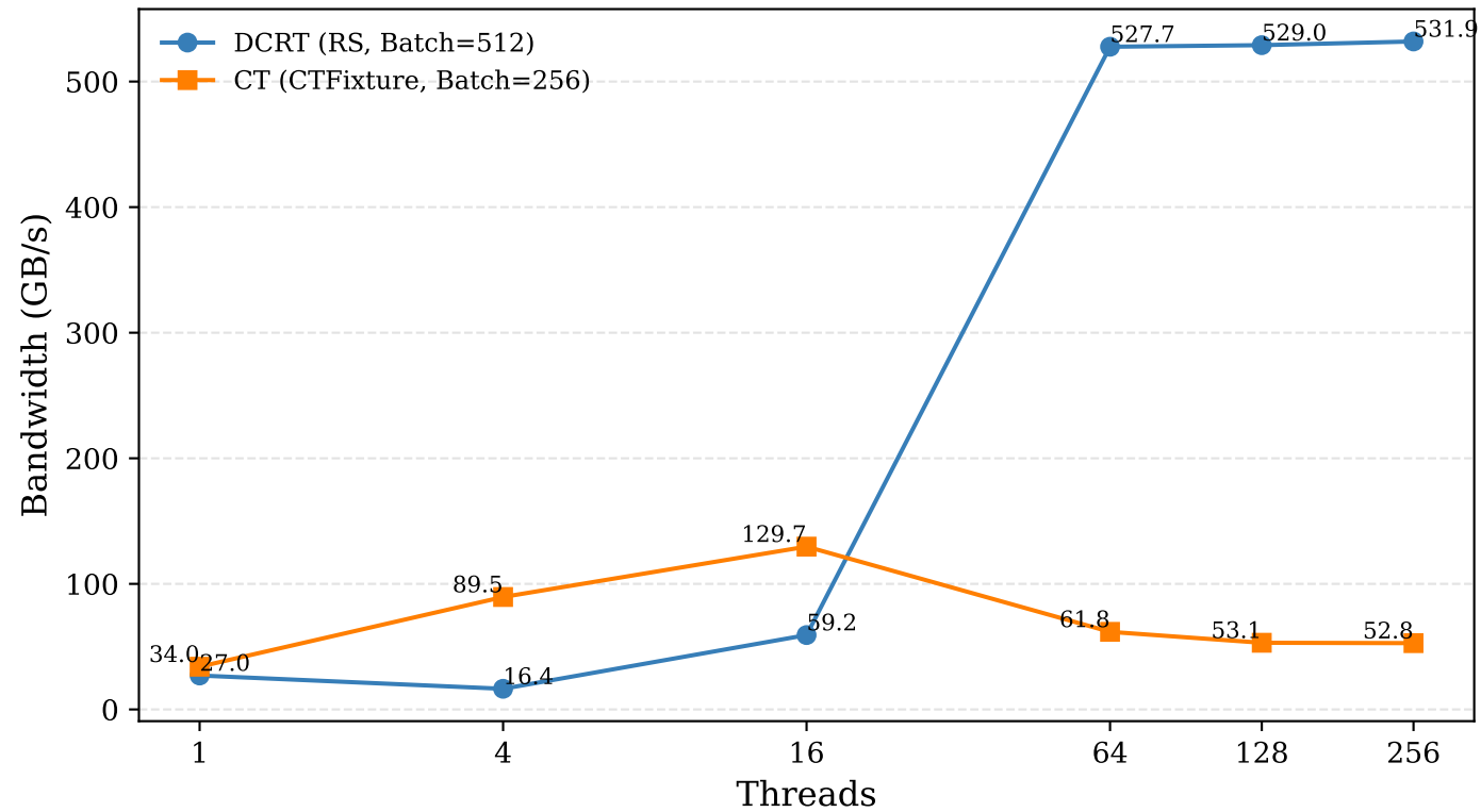
ADD Kernel: Bandwidth vs Threads [N=131072, L=40]
