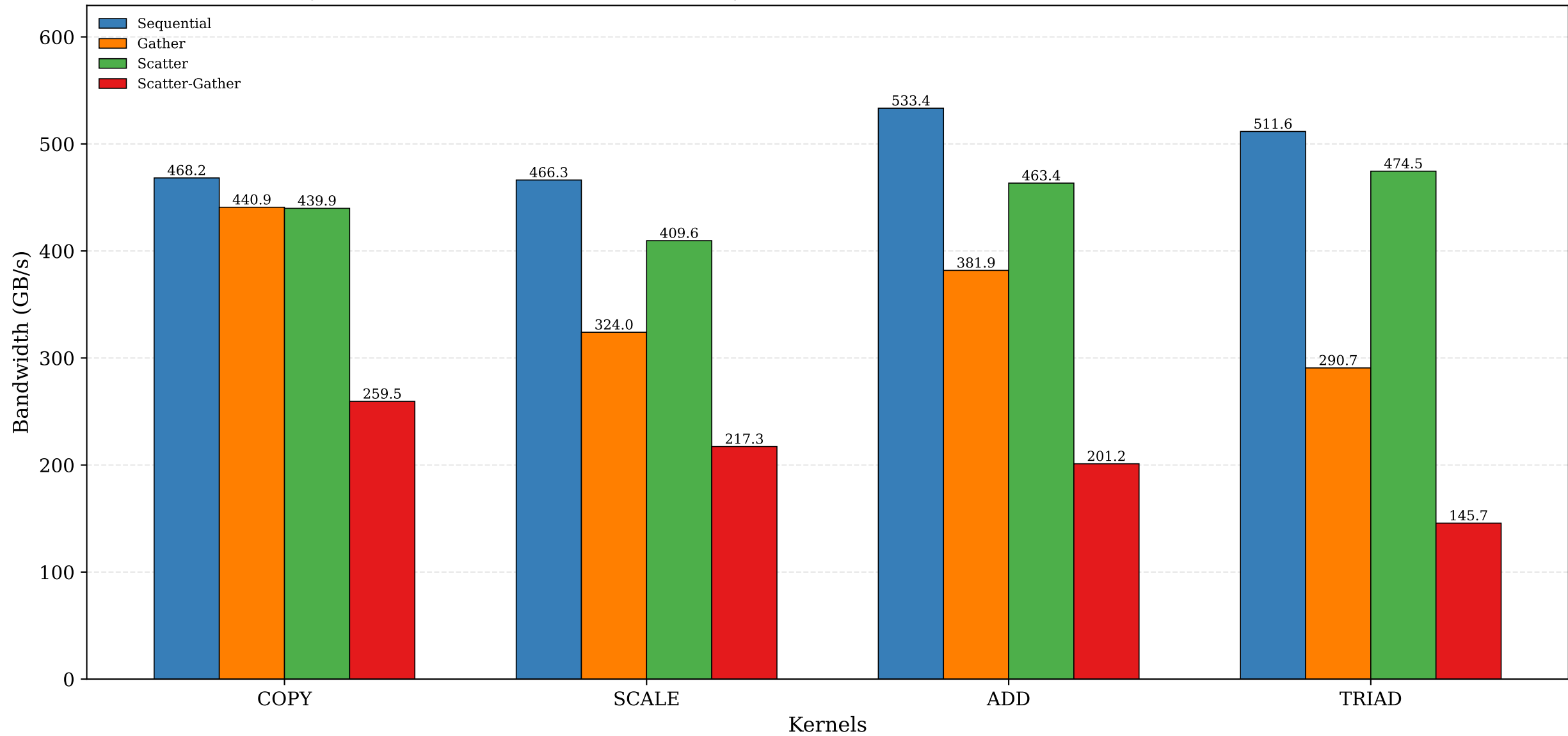
DCRTPoly Backend: Bandwidth Across Memory Access Patterns (Coeff mode) [N=131072, L=40, Batch=512]
