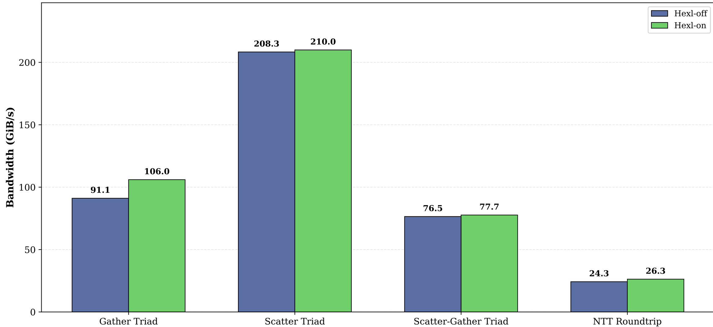
HEXL-off vs HEXL-on Bandwidth Comparison (GiB/s) N=131072, L=40
