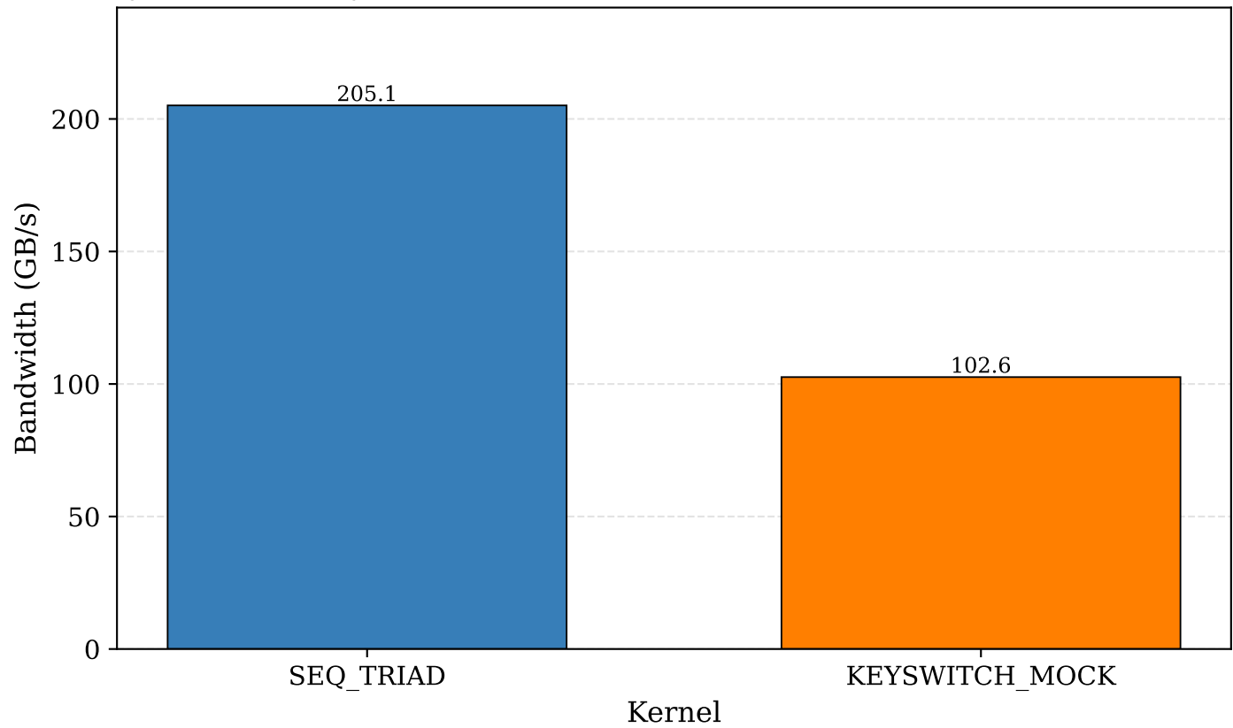
DCRTPoly Backend: Keyswitch Mock vs Sequential Triad [N=65536, L=20, Batch=100]
