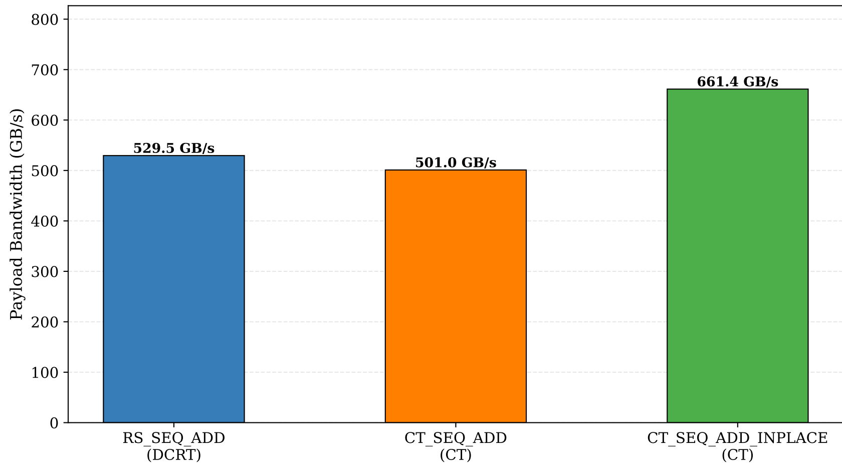
ADD Kernel: Software Overhead Comparison (256 threads, Batch=256) N=131072, L=40
