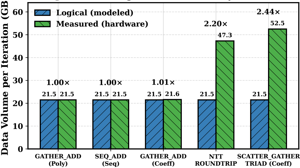
DRAM Amplification: Logical vs Measured Byte Volume (Write)
