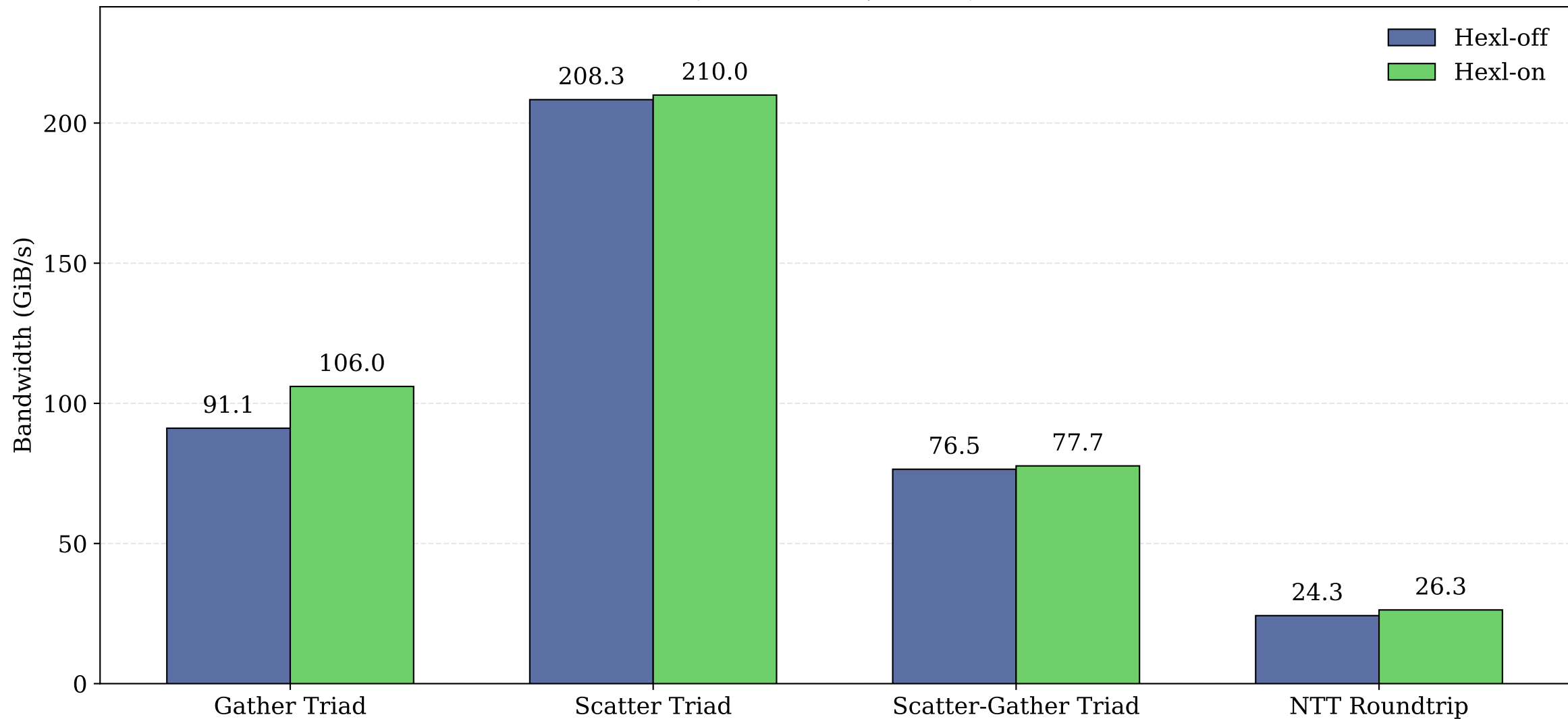
DCRTPoly: HEXL-off vs HEXL-on Bandwidth Comparison (GiB/s) (N=131072, L=40)
