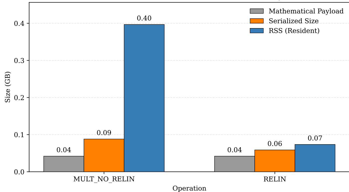
Estimated vs Serialized vs Resident (RSS) Payload
