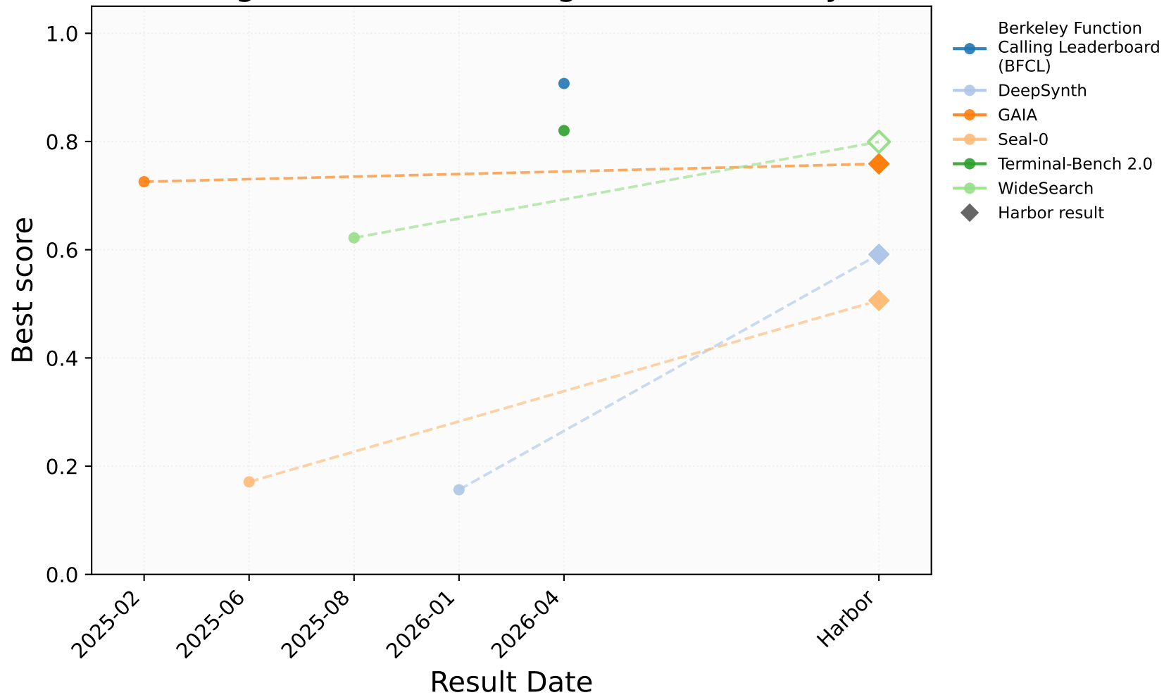
Score Progress Over Time: Agents, Tools & Systems
