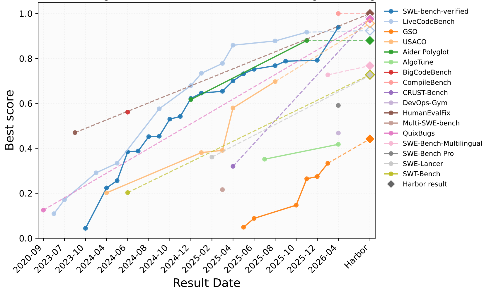
Score Progress Over Time: Software Engineering
